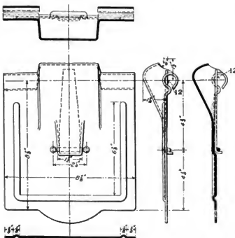
Figs. 4497-4501. Davis Pressed Steel Journal Box Lid. Davis Pressed Steel Co.
